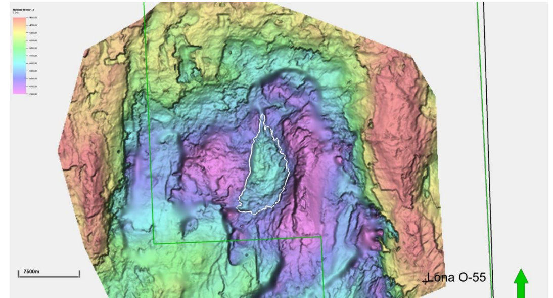
Top Jurassic Depth Structure
